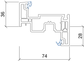
Anta Minimal Standard Boot Leaf
