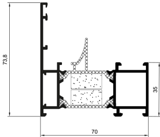
Telaio piano anta a scomparsa Flat door frame
